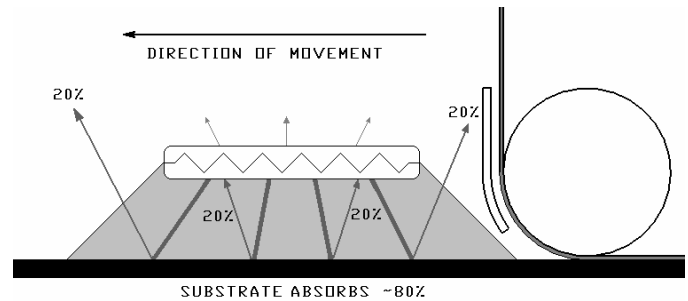
Figure 4. Undesirable Reflected IR and Waste Heat
