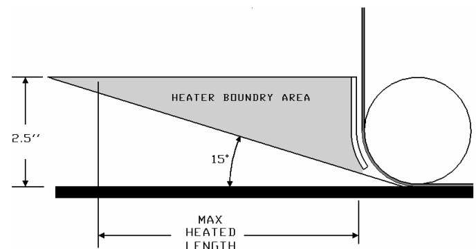
Figure 1. Heater Geometry Constraints
