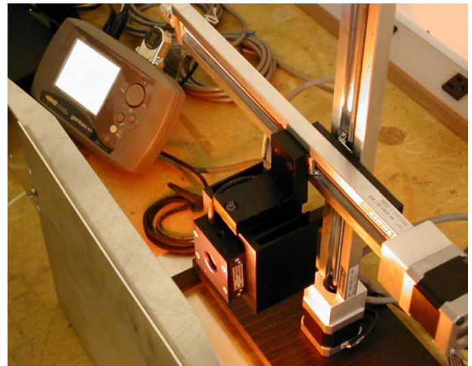
Figure 7 Power Meter on X/Y Stage Measuring Irradiance
